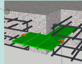
Internal Construction Joint
