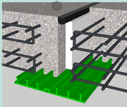
External Expansion Joint
