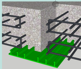
External Construction Joint
