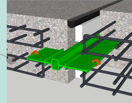
Internal Expansion Joint
